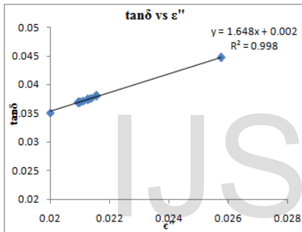
Graph (5) Tangent loss versus Dielectric loss
