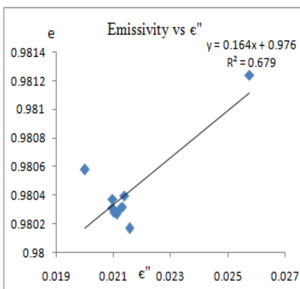
Graph (7) Emissivity versus Dielectric loss
