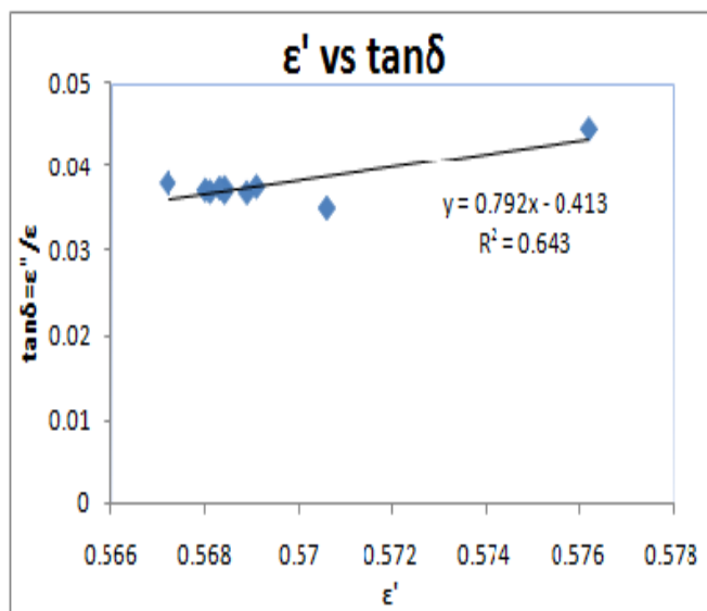
Graph (1) Dielectric constant verses Tangent loss
