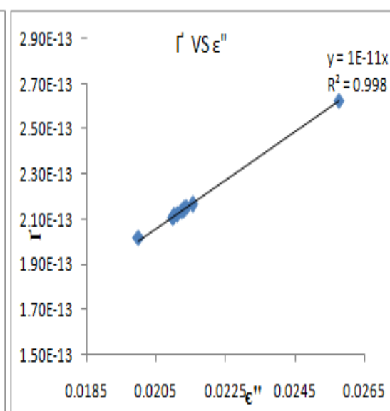
Graph (8) Relaxation time versus Dielectric loss
