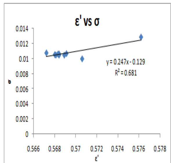
Graph (2) Dielectric constant verses Conductivity
