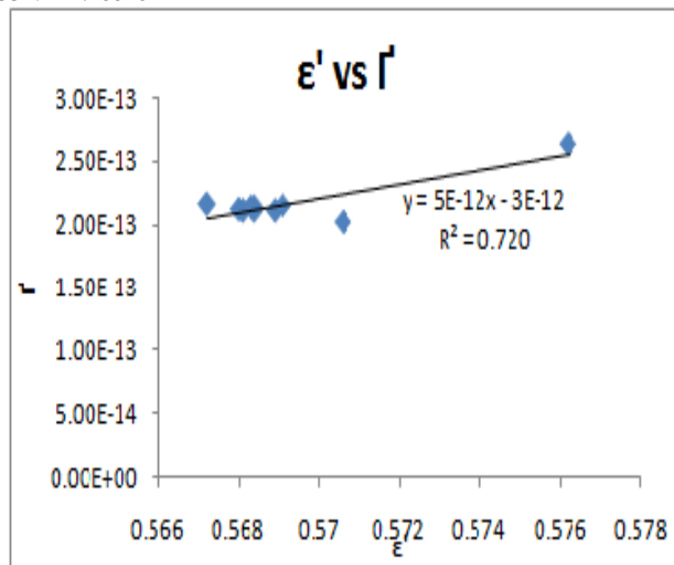
Graph (3) Dielectric constant versus Relaxation time
